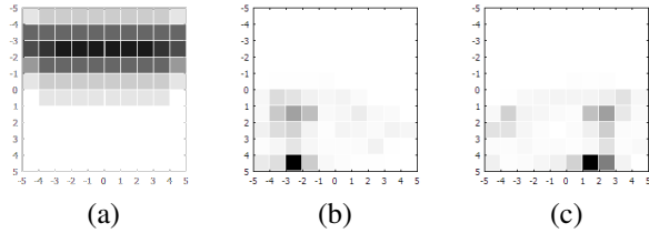
Fig. 6. 2D Look-up tables used for the computation of P(l_i|F) in Equation (7). (a) for faces, (b) for left hands, (c) for right hands.
