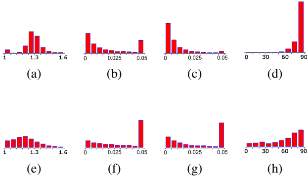
Fig. 5. 1D Look-up tables used for the computation of Equation (7). (a): P(r_l|F = \text{face}) , (b): P(u_l|F = \text{face}) , (c): P(v_l|F = \text{face}) , (d): P(\theta_l|F = \text{face}) , (e): P(r_l|F = \text{hand}) , (f): P(u_l|F = \text{hand}) , (g): P(v_l|F = \text{hand}) , (h): P(\theta_l|F = \text{hand}) .
